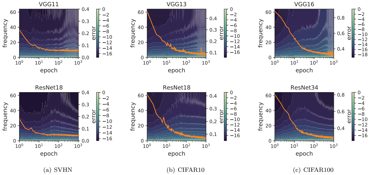
Figure 1: Models trained on SVHN, CIFAR10 and CIFAR100 with 0% label noise. The heat map with contour lines depicts R_k which is calculated on the training set, where k denotes the “frequency”.
