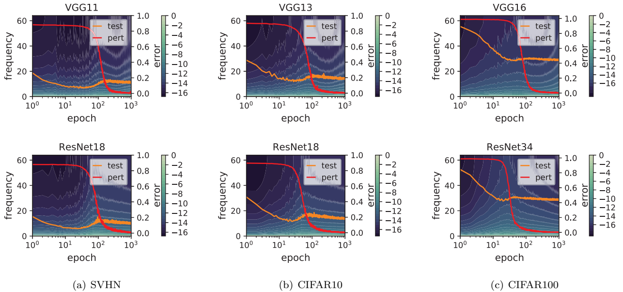
Figure 2: Models trained on SVHN, CIFAR10 and CIFAR100 with 20% label noise. The heat map with contour lines depicts R_k which is calculated on the training set, where k denotes the “frequency”.
