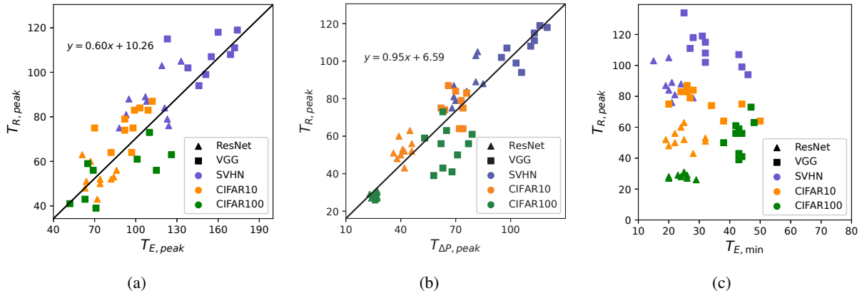
Figure 6: (a) T_{R,peak} w.r.t. T_{E,peak} ; (b) T_{R,peak} w.r.t. T_{\Delta P,peak} ; (c) T_{R,peak} w.r.t. T_{E,min} . The colors represent different datasets, whereas the shapes indicate different categories of DNNs, e.g., green squares represent VGG on CIFAR100. The black line is fitted by linear regression. Each experiment was repeated five times. The Pearson correlation coefficients for (a) and (b) are 0.88 and 0.92, respectively.
