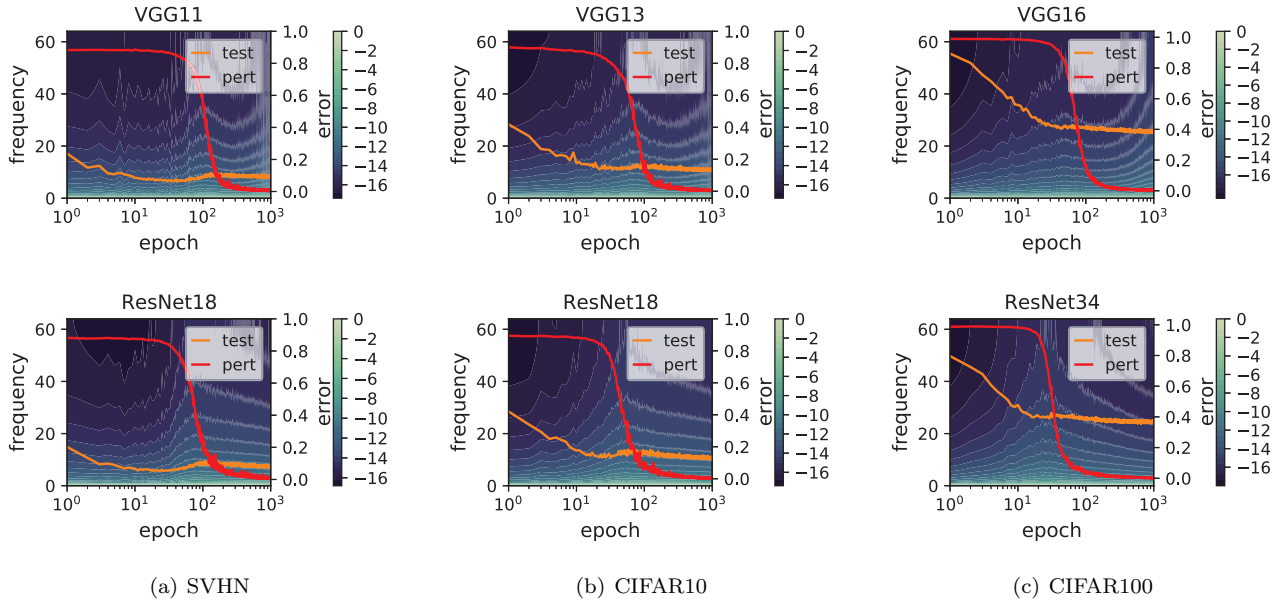
Figure 3: Models trained on SVHN, CIFAR10 and CIFAR100 with 10% label noise. The heat map with contour lines depicts R_k , which is calculated on the test set , where k denotes the “frequency”.
