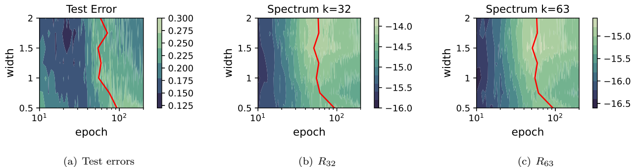
Figure 4: Test error and R_k w.r.t. model width. The original model is ResNet18 trained on CIFAR10 with 20% label noise. The red lines depict the exact positions of peaks of test errors and R_k .
